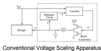
Conventional Voltage Scaling Apparatus
