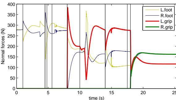
Fig. 10. Experiment B: Vertical forces distribution.
