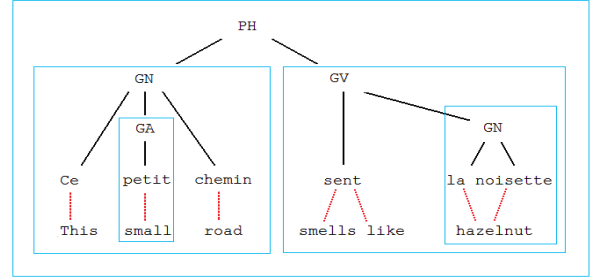
Fig. 2. Selecting Sub-sentential Rules
