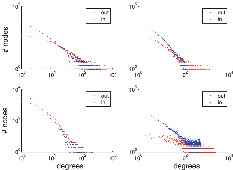
Fig. 5 Distributions for 4 different parameter sets on the adopted model. a Top left \alpha = 0.018 , \beta = 0.102 , \gamma = 0.88 , \delta_{in} = 1 , \delta_{out} = 2 . b Top right \alpha = 0.018 , \beta = 0.102 , \gamma = 0.88 , \delta_{in} = 5 , \delta_{out} = 1 . c Bottom left \alpha = 0.102 , \beta = 0.238 , \gamma = 0.66 , \delta_{in} = 1 , \delta_{out} = 3 . d Bottom right \alpha = 0.001 , \beta = 0.009 , \gamma = 0.99 , \delta_{in} = 1 , \delta_{out} = 1
