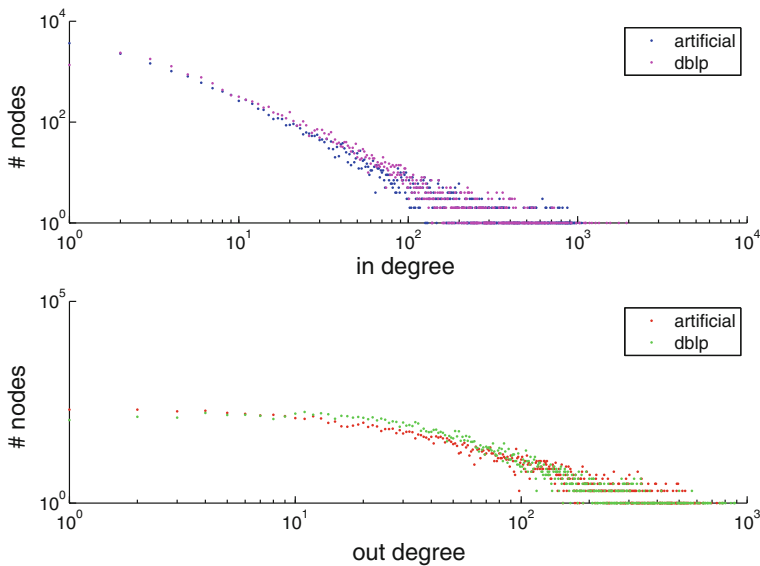
Fig. 6 Comparison of the distributions for the in/out degrees between the chosen parameters ( \alpha = 0.011 , \beta = 0.031 , \gamma = 0.958 , \delta_{\text{in}} = 2 , \delta_{\text{out}} = 5 ) and the DBLP graph
