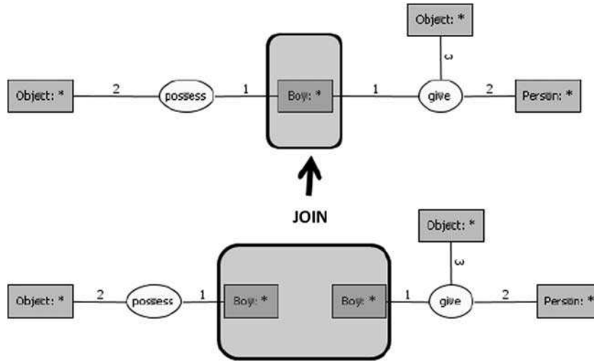
Figure 19 Disjoint sum
