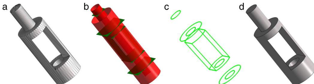
Fig. 18. B-Rep reconstruction for CylindricalAdaptor : (a) 3D mesh: (268 vertices and 540 triangles), (b) Extracted geometric primitives (3 cylinders and 7 planes), (c) Reconstructed wires and (d) the final B-Rep model.
