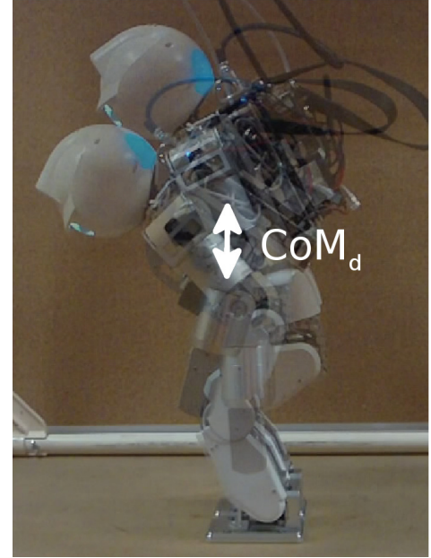
Fig. 8: Squat-like motions.
