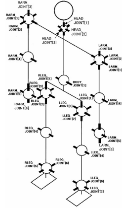
(b) HOAP-3 kinematics model
