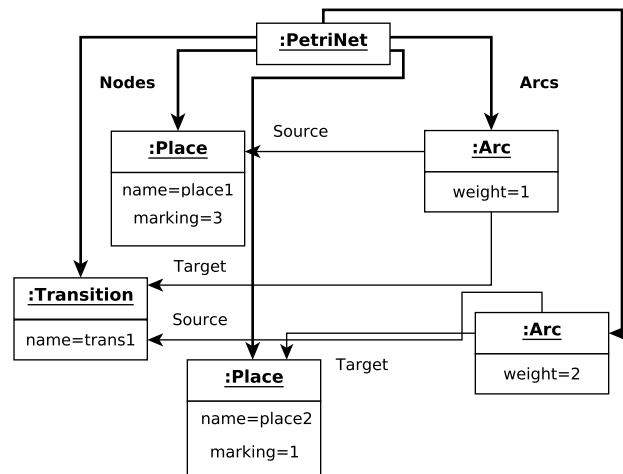
Figure 4. A model for a Petri net, seen as an instance of the Petri net metamodel of Figure 3.
