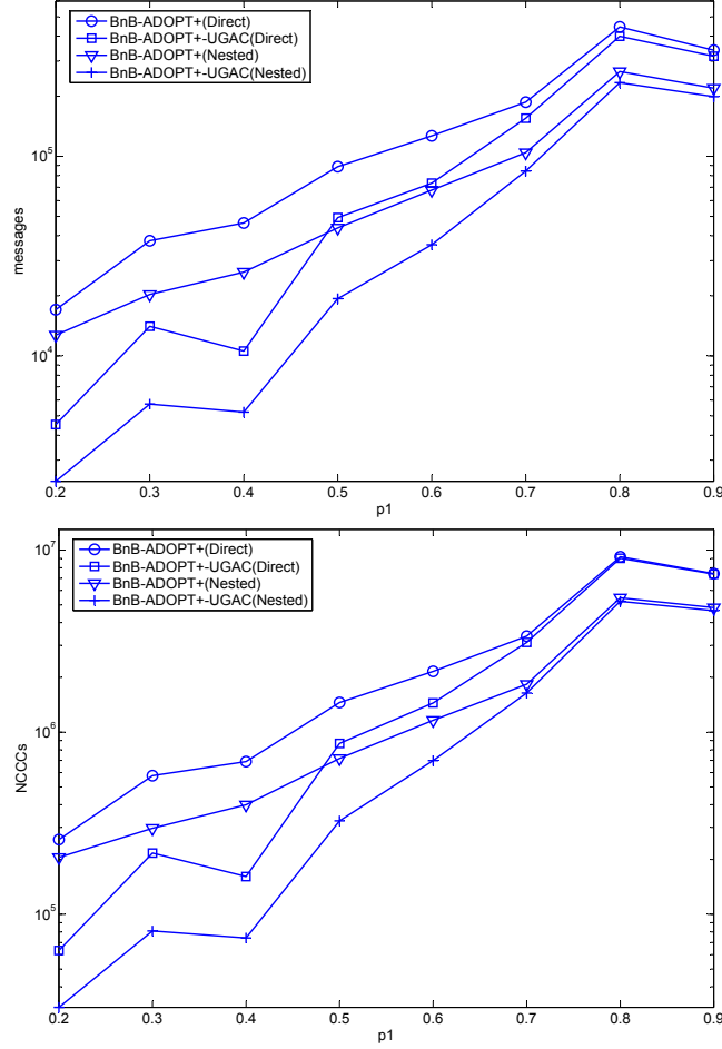
Figure 21: Experimental results of random DCOPs including soft-at-most global cost functions with the violation measure \mu_{var} .
