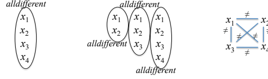
Figure 4: Representations considered for the global constraint all\text{-}different(x_1, x_2, x_3, x_4) : (left) direct representation, (center) nested representation, (right) binary representation.
