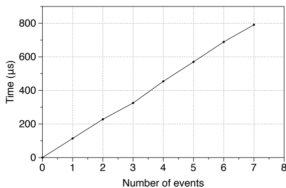
Figure 12. Performance of the Omega Algorithm
