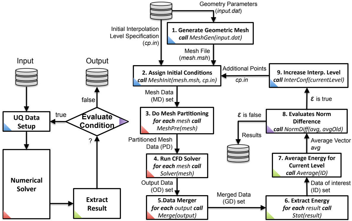
Figure 2. Iterative UQ workflow
