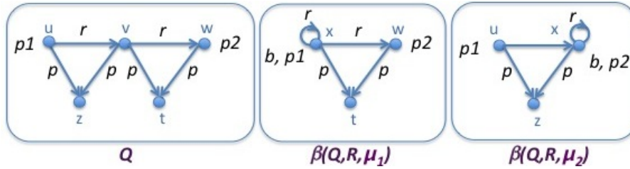
Figure 4: The queries in Example 10
