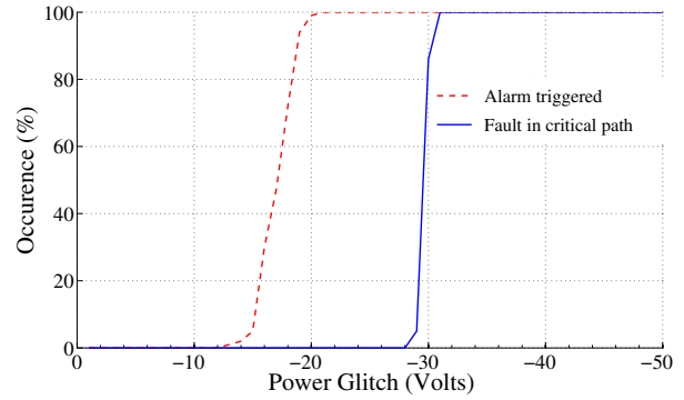
Fig. 3. Detection of power supply glitches.
