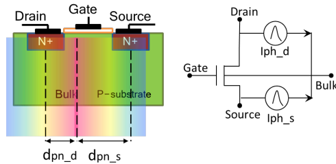
Figure 3. Simple electrical model for a large spot laser-induced fault
