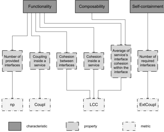
Figure 2. Refinement model of service characteristics.
