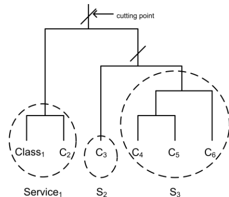
Figure 3. Dendrogram with set of services.
