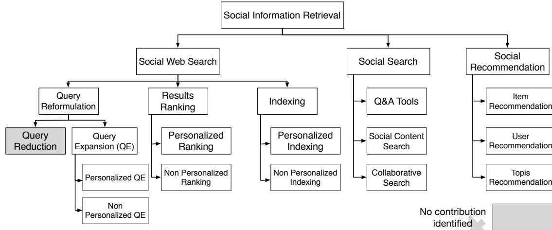
Figure 2: A taxonomy for Social Information Retrieval Models.
