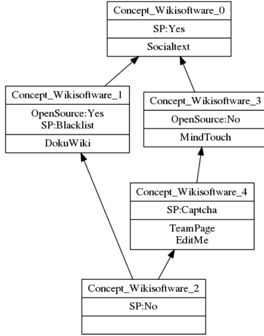
Fig. 8. Concept lattice of Wikisofwares, step 0
