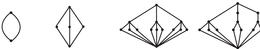
Fig. 4. The sets \mathcal{H}_0 , \mathcal{H}_1 , and part of \mathcal{H}_2 .
