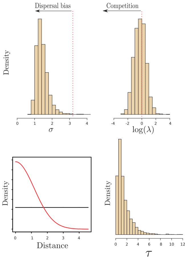
FIGURE 5. Posterior distribution of parameter estimates for the Banza data set. The two histograms at the top correspond to the posterior distributions of the parameters \lambda and \sigma , measuring competition intensity and dispersal bias, respectively. The dotted lines indicate thresholds below which competition occurs and dispersal is biased toward short distances. The histogram at the bottom gives the posterior distribution of \tau , the overall dispersal rate parameter. The densities on the bottom-left corner are that of a uniform (in black) in [0, 4.56] , where 4.56 is the mean distance between islands (the unit is not relevant) and that of a normal density (in red) with mean 0 and variance equal to the posterior median of \sigma , truncated to [0, 4.56] .
