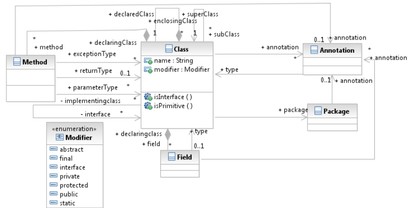
Fig. 3 Java metamodel
