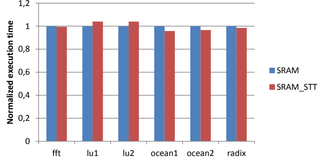
Fig. 2. Execution time on four-core architecture (Normalized to execution time of “SRAM” scenario)
