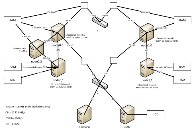
Fig. 5: The HLRS cloud platform
