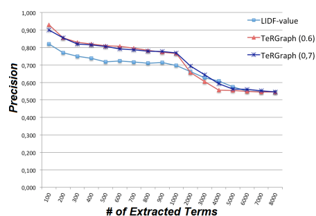
Fig. 10 Precision comparison of LIDF-value and TeRGraph
