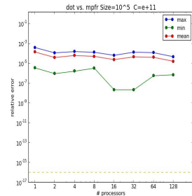
Figure 2: Relative differences in dot product algorithms (min, max, mean). X-axis: p processors (1...128). Horizontal dotted line: \forall C \approx 10^{11} and n = 10^5
