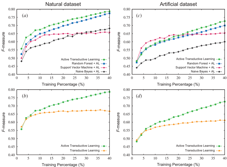
Figure 2. Classification results varying the percentage of training examples between 2% to 40% for: the Natural (left side) and the Artificial (right side) data sets. (a) All classification methods coupled with AL over the Natural data set. (b) Our framework with and without AL over the Natural data set. (c) All classification methods coupled with AL over the Artificial data set. (d) Our framework with and without AL over the Artificial data set.
