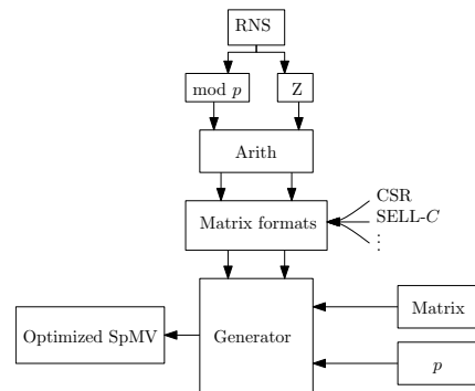
Fig. 1. Generator workflow
