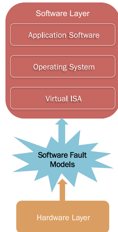
Fig. 6. Software stack.
