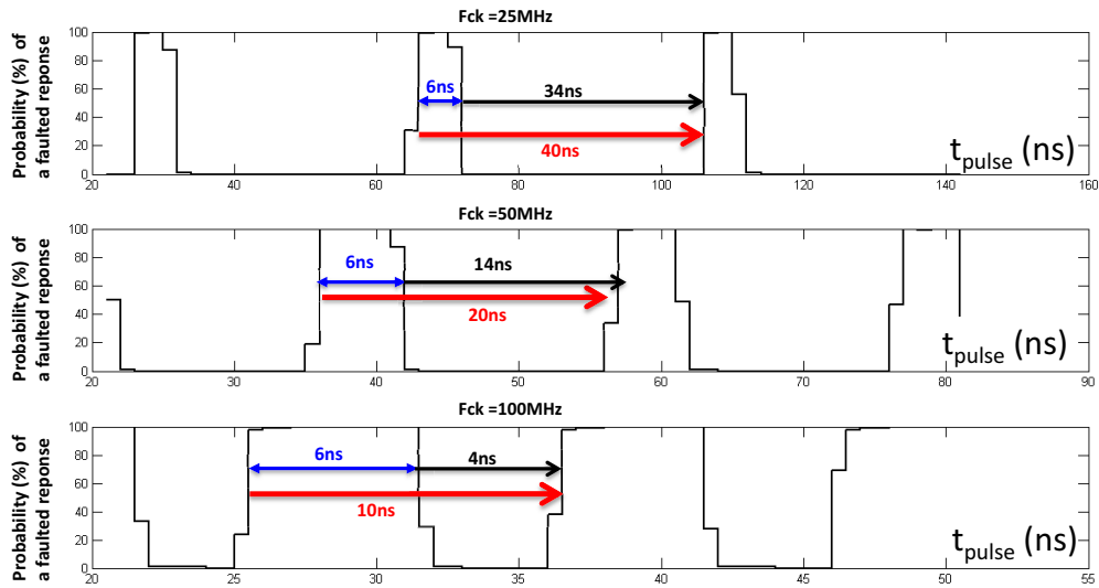
Figure 8. Evolution of the probability to induce a fault into the hardware AES mapped onto a spartan3-1000 wrt t_{pulse}
