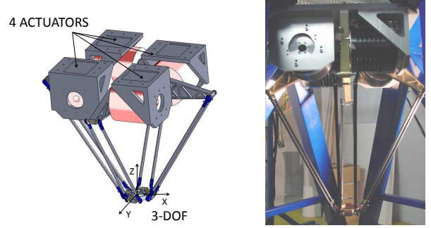
Fig. 1. Views of the R4 parallel manipulator: Schematic view of the CAD design (left), side view of the robot prototype (right)
