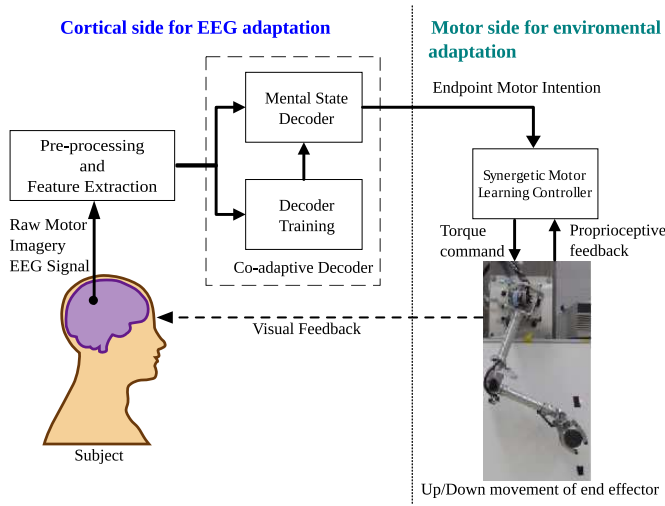
Fig. 1. BMI paradigm employed in this paper for simultaneous control of multi-DOFs robot using adaptive left-right MI decoder and synergetic motor learning for peripheric joint redundancy management. The black dots indicate the targets for the subjects in the vertical plane.
