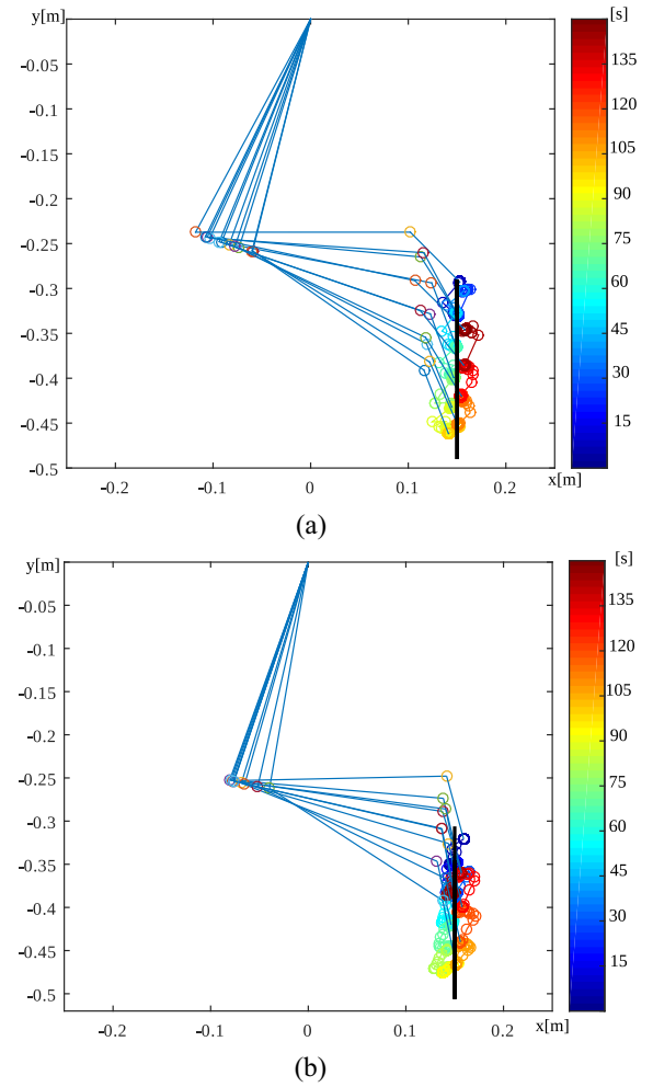
Fig. 10. Trace of the movement of the robot arm during simultaneous multi-DOF robot control which is driven by the subject motor intention through co-adaptive BMI. The robot is holding (a) 300 g load, (b) 600 g load. The joint angle variance on shoulder and wrist for the heavier weight condition has become half compared to lighter weight condition.
