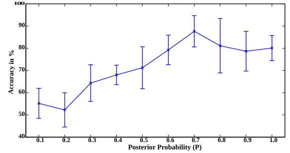
Fig. 7. Average accuracies obtained over nine subjects, while changing the limiting posterior probability from 0.1 to 1.0.
