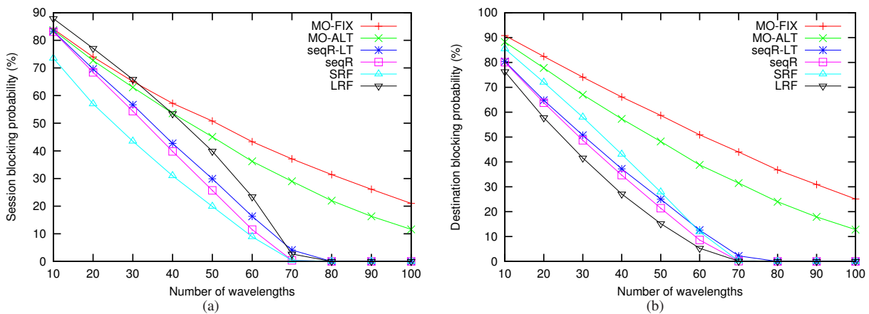
Fig. 5: Performances of the strategies on US Longhaul network with S = 6 random MC-OXCs, |R| = 200 requests: a) SBP vs. Number of wavelengths; b) DBP vs. Number of wavelengths
