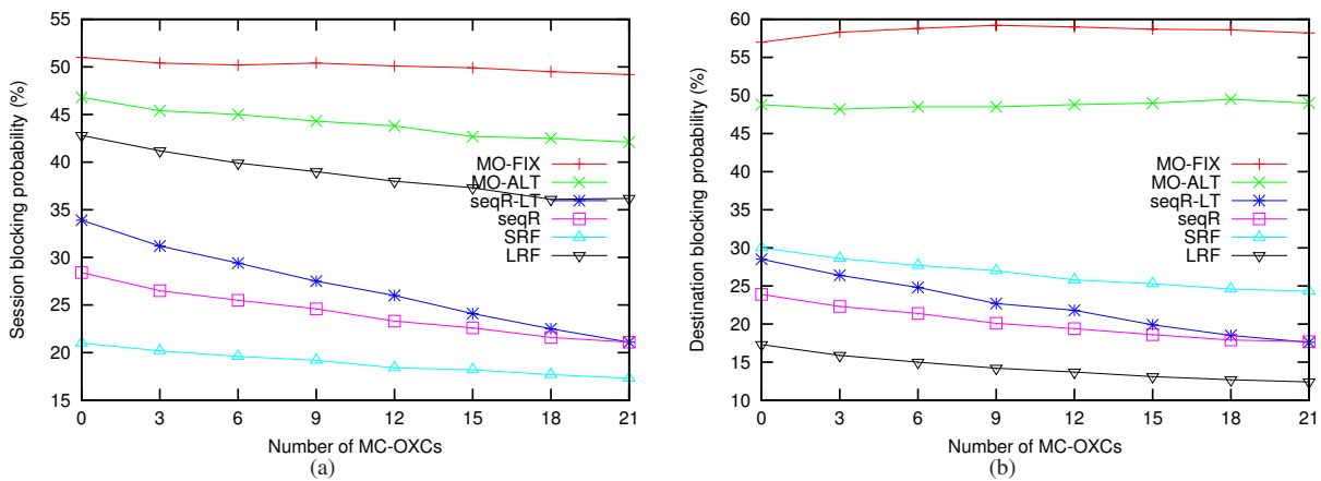
Fig. 6: Performances of the strategies on US Longhaul network with |R| = 200 requests, |W| = 50 wavelengths: a) SBP vs. Number of MC-OXCs; b) DBP vs. Number of MC-OXCs
