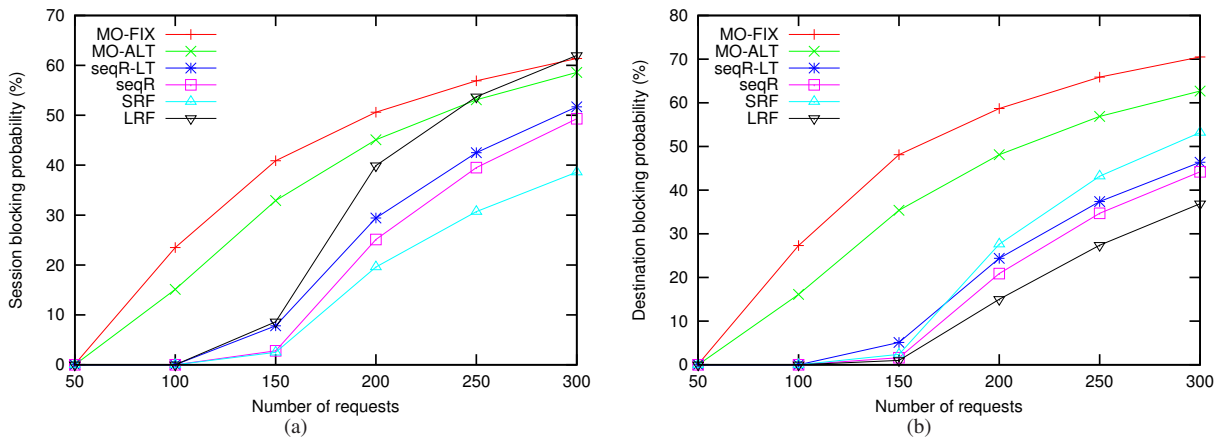
Fig. 7: Performances of the strategies on US Longhaul network with S = 6 MC-OXCs, |W| = 50 wavelengths: a) SBP vs. Number of requests; b) DBP vs. Number of requests
