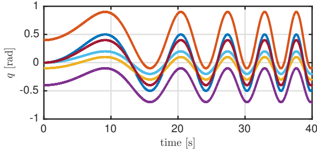
Fig. 6. Joint trajectory used for estimating backlash and friction coefficients.
