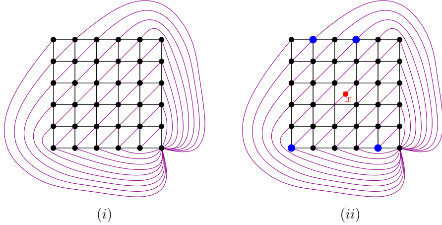
Figure 6: The leftmost graph is \Gamma_6 . The insulation of x in the rightmost graph is equal to 2 (the terminals are the blue vertices).
