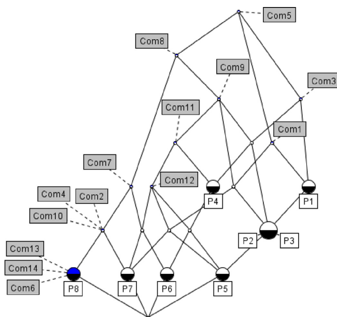
Fig. 12. The concept lattice of MM architecture configurations.
