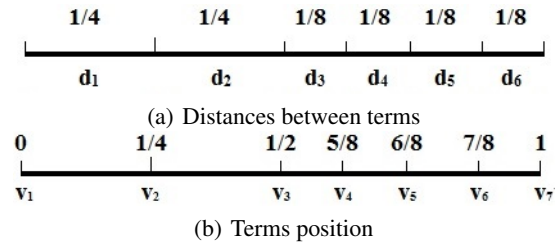
Figure 6 – Algorithm inputs
