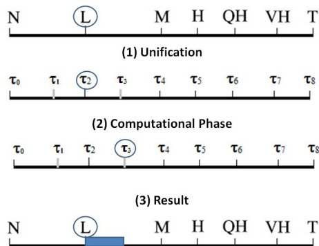
Figure 2 – Management of unbalanced linguistic term set
