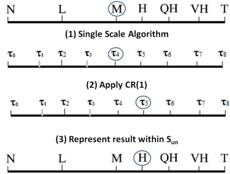
Figure 11 – The process of applying CR (1) to relevance degree M
