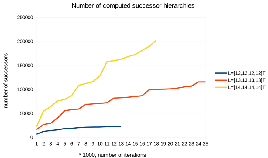
Figure 11. he evolution of the number of computed hierarchies in the NTT example.
