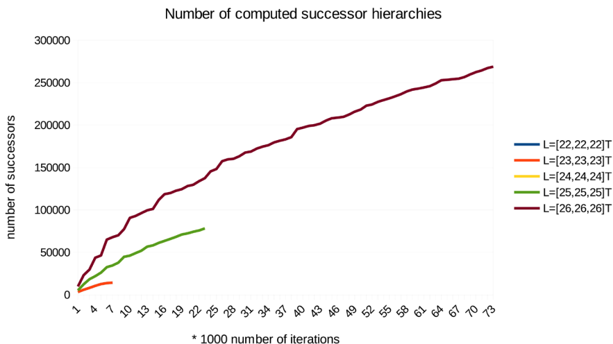
Figure 9. The progression of the number of computed hierarchies in the first example.
