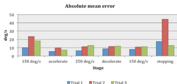
Figure 6. Reference tracking results
