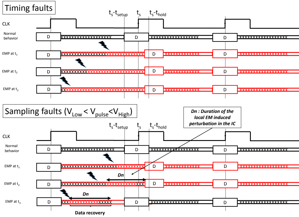
Fig. 15 The Comparison of timing faults and sampling faults
