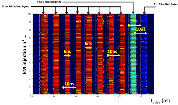
Fig. 11 Number of faulted bytes wrt to t_{pulse} for the 100 plaintexts processed by the AES
