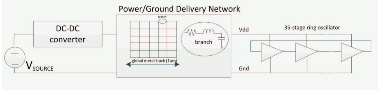
Figure 1. Overall description of analysis framework for investigating on-chip DC-DC conversion.
