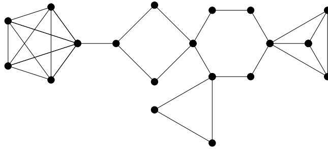
Fig. 1. A clique-cactus graph.
