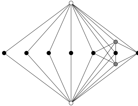
Fig. 5. The graph W_{4,3} . Poles are drawn in white and semipoles in gray.
