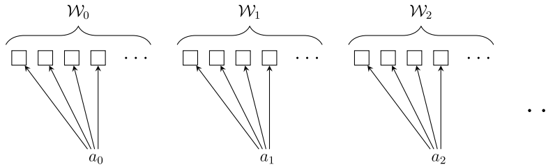
Fig. 4. The situation described in Lemma 11. Arrows are directed towards larger elements.
