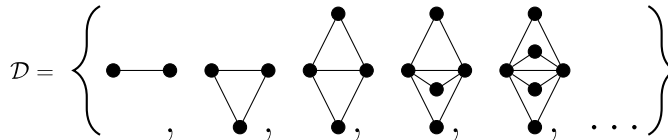
Fig. 2. Graphs of \mathcal{D} .
