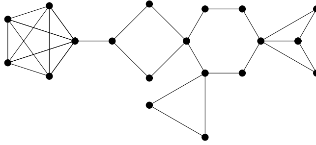
Fig. 1. A clique-cactus graph.
