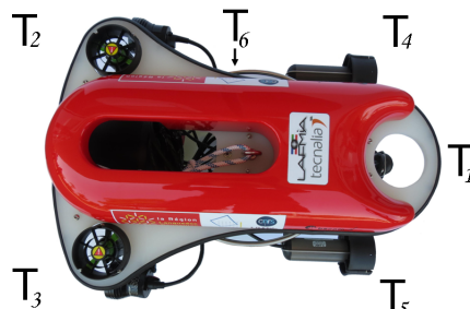
Figure 2: L2ROV: View of forces generated by the thrusters to perform the translational and rotational motions.
