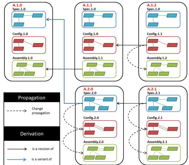
Figure 1. Versioning Architectures
