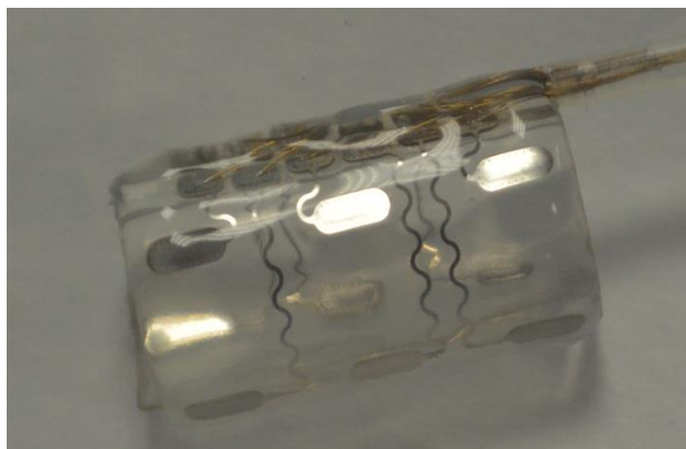
Fig 1. 12-poles multipolar cuff electrode
