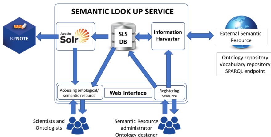
Fig. 1. Proposed architecture and data flow in EUDAT's Semantic Lookup Service
