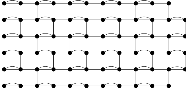
Fig. 1. The graph \widehat{W}_5 .
