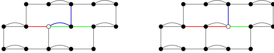
Fig. 3. Swapping branch vertices.
