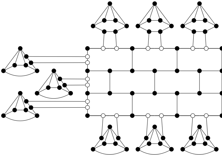
Fig. 5. The host graph G .
