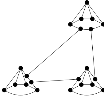
Fig. 4. A biconnected graph H for which \mathcal{I}(H) does not have the v/e-E&P property.
