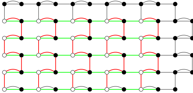
Fig. 2. Finding \Gamma_5 as a strong immersion in \widehat{W}_5 . (For interpretation of the references to colour in this figure legend, the reader is referred to the web version of this article.)
