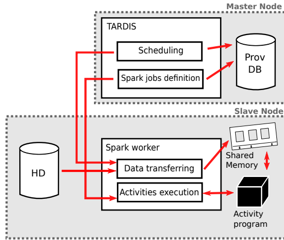
Fig. 1. TARDIS architecture.
