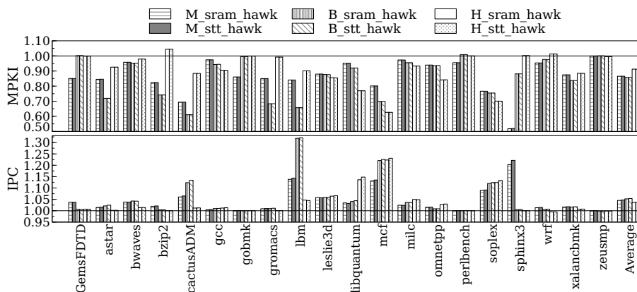
Fig. 6: Performance impact of Hawkeye normalized to LRU
