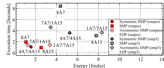
(j) lud (gem5/McPAT simulation)
